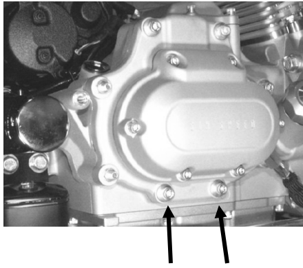
Photo 1: Remove Trans Bolts
